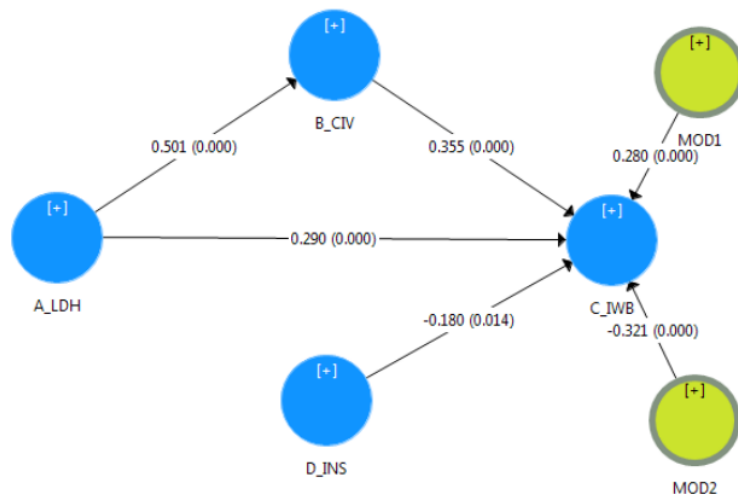
Figure 3. SmartPLS 3 result for structural model
