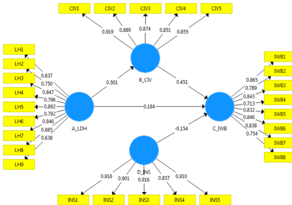
Figure 2. SmartPLS 3 result for measurement model
