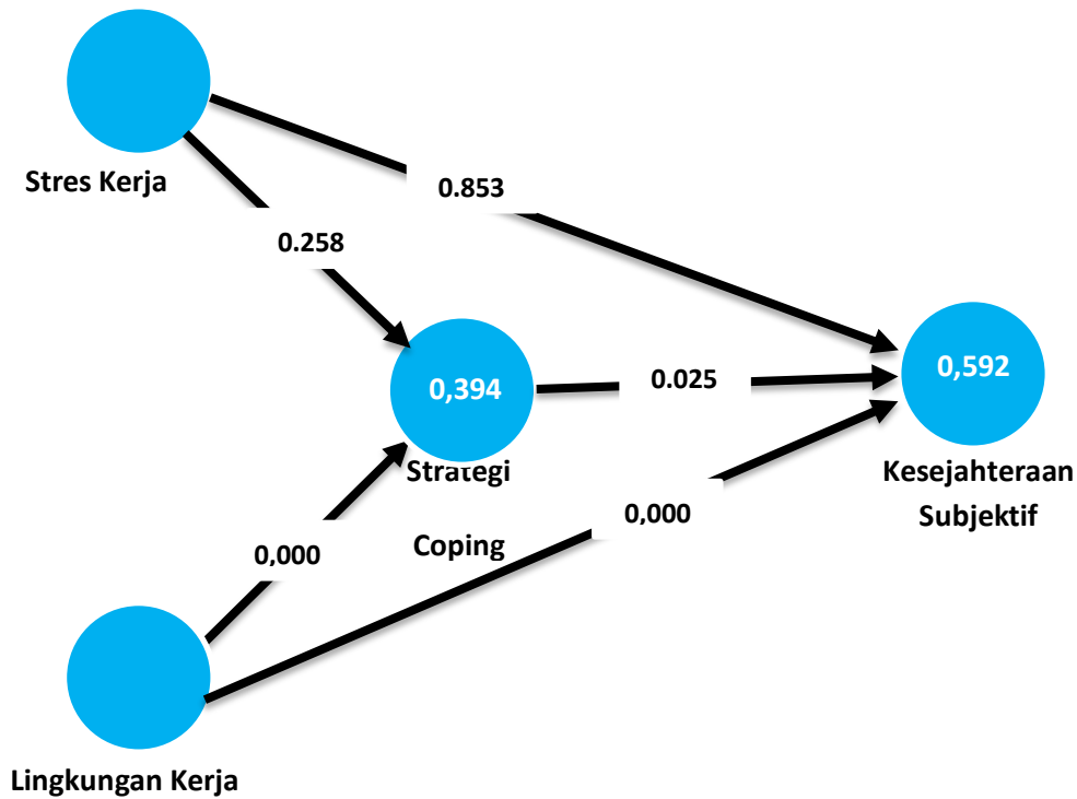
Gambar 1. Model Partial Least Square
