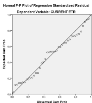
Gambar 1. Normal P-Plot
