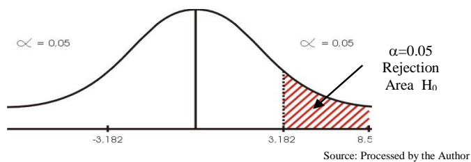
Fig. 1. Normal distribution.
